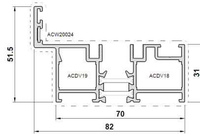
Outer Frame and Standard Threshold
