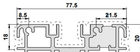
Low Threshold Open Out
