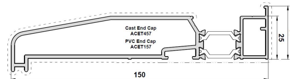
150mm Cill
