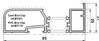
85mm Cill
