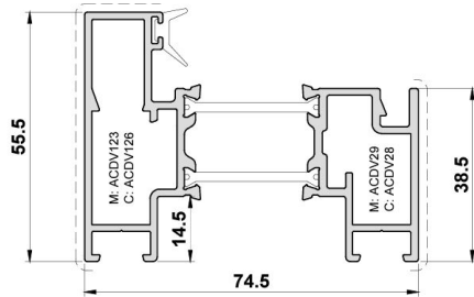
Sash with Quick Bead
