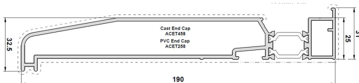
190mm Cill
