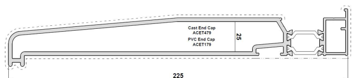
225mm Cill
