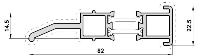
Horizontal Coupler
